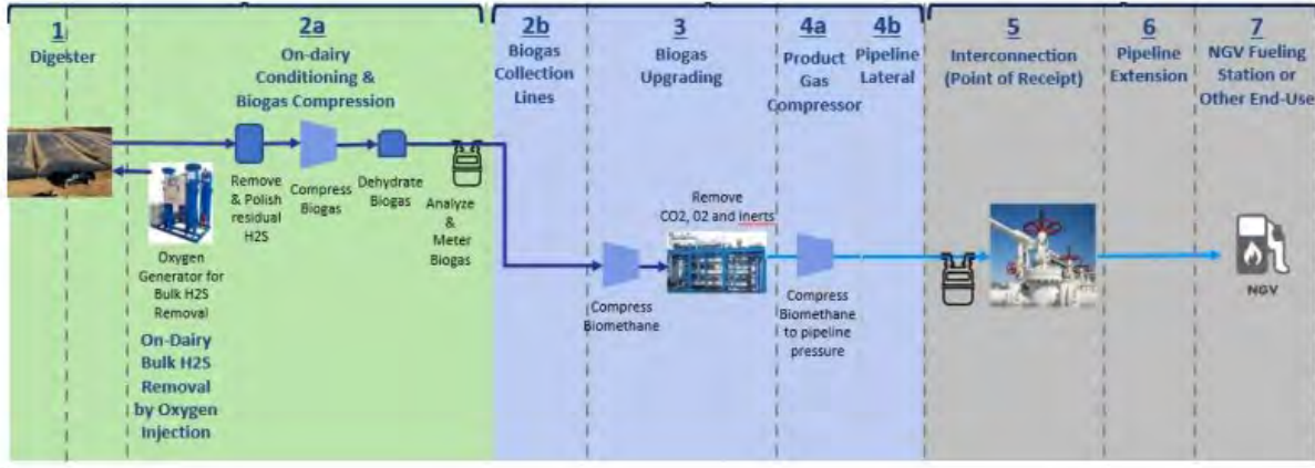
Figure 1: Process to Convert Dairy Biogas into R-CNG
