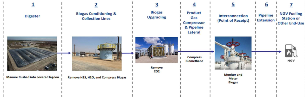
Figure 1: Process to Convert Dairy Biogas into R-CNG
