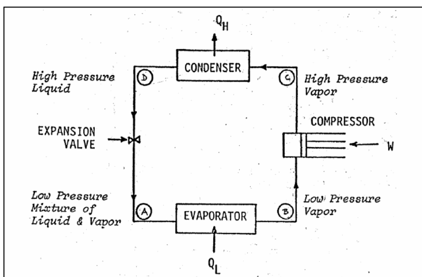
Figure 3: Schematic drawing of a vapor compression chiller cycle. This chiller is similar to absorption and adsorption chillers, which use heat, rather than a mechanical system, to compress the vapor.
