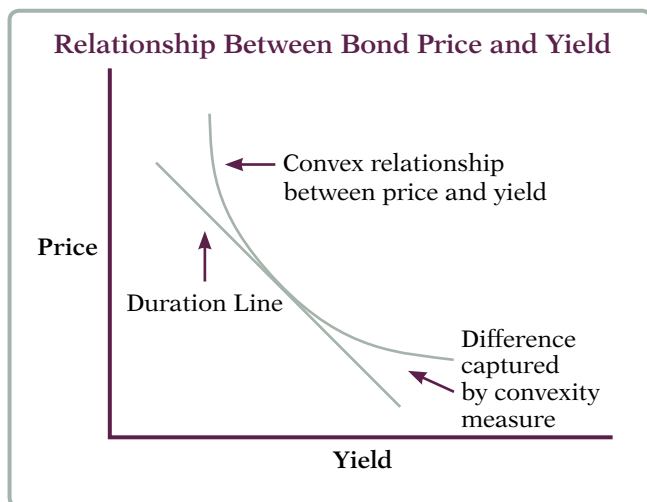
Figure 6 – Convexity
